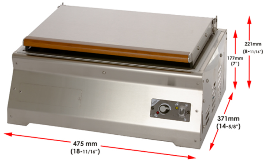
85NDP stove/heater
